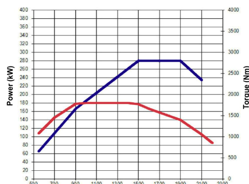
Cursor 13 - 380 HP (283 kW)
